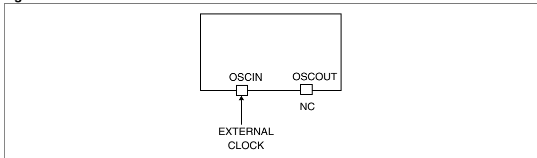
Figure 13. External clock source connections
